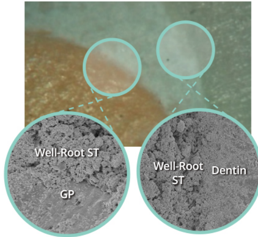
Optical microscope image of microleakage test (dye penetration test) ; No dye penetration
